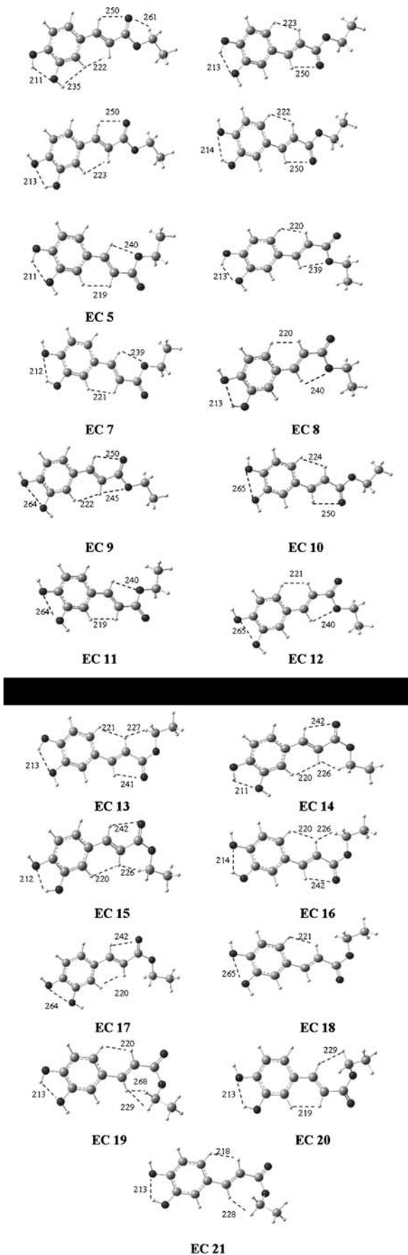
Fig. 5 Representation of the several conformers calculated for EC displaying (C)H \cdots O and (O)H \cdots O intramolecular interactions. B3LYP/6-31G** level of calculation. Intramolecular distances are represented in pm
